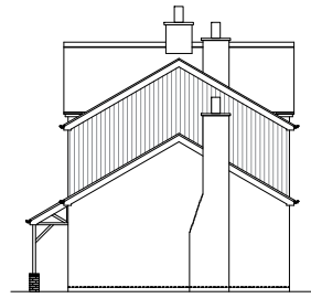
SIDE ELEVATION 2
