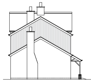
SIDE ELEVATION 1
